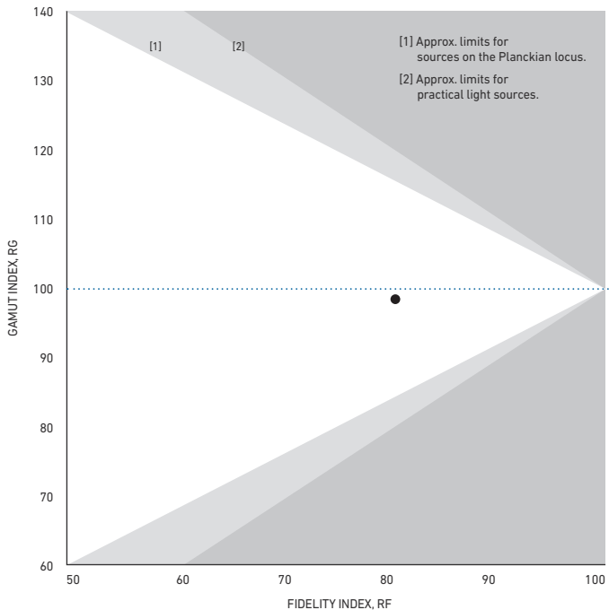
IES TM-30-15
